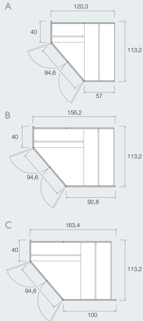
2 DOORS CORNER CABIN WITH FIXED 40 CM. SIDE
