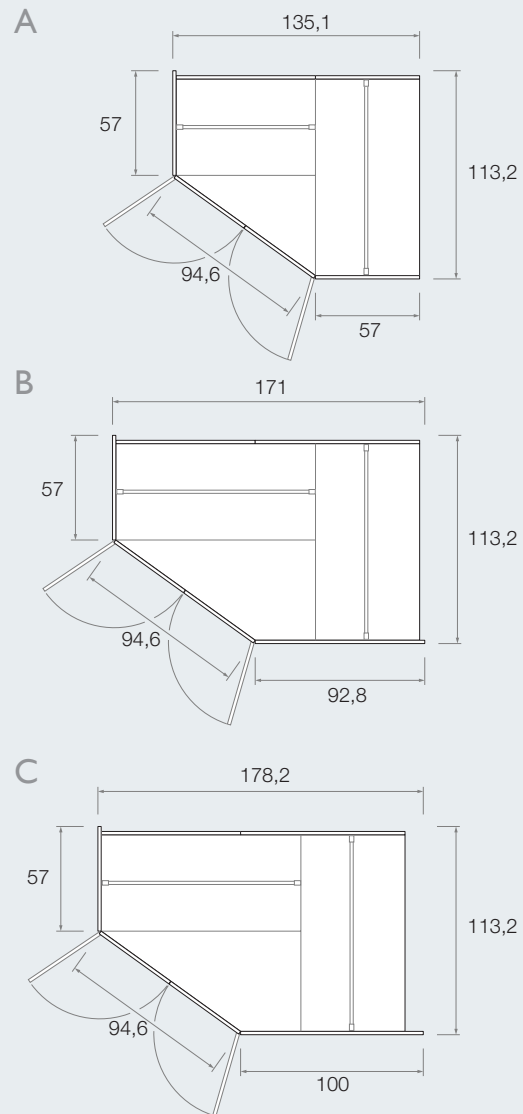
2 DOORS CORNER CABIN
